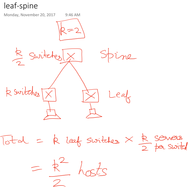
Figure 1: 2 layer leaf-spine topology with k=2 port switches
